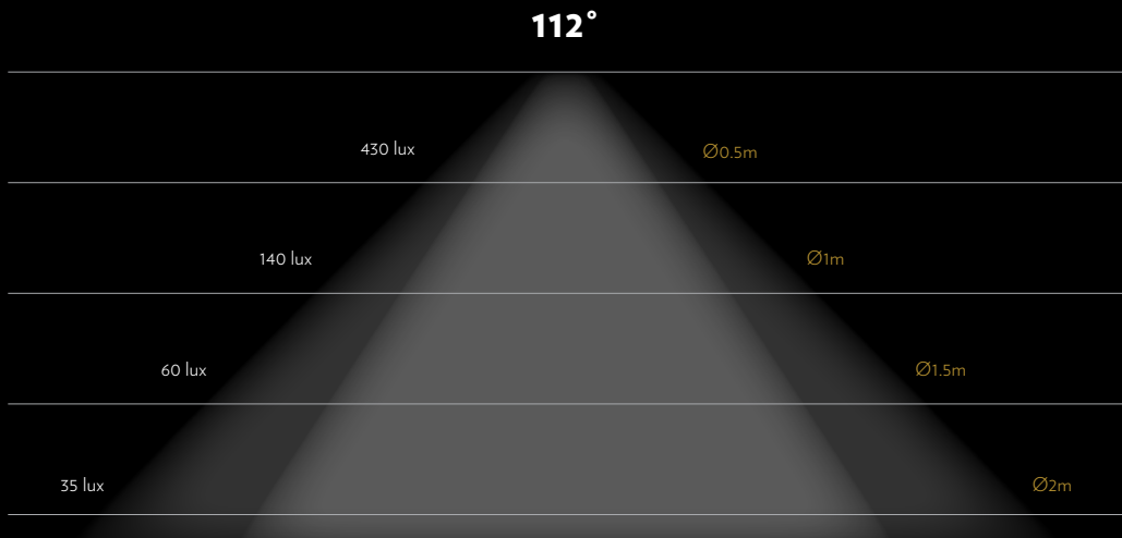
L-MTBA-450 Lightbar 7W (18")
