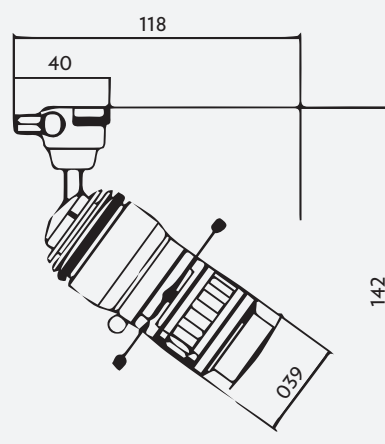
L-MTFS-22 6W - Quadri Framing Shutter Spotlight
