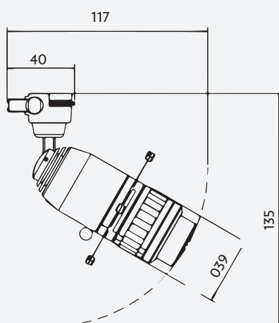
L-MTFS-02 3W - Quadri Framing Shutter Spotlight
